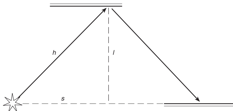
Figure 2 Path of light viewed from the platform.
