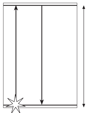
Figure 1 Light clock as viewed by observer on the train.
